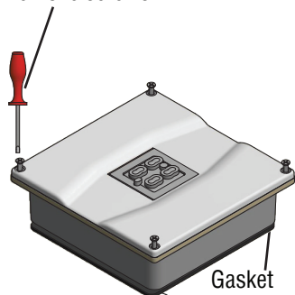
Figure 1 Remove screws
