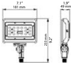
Knuckle
