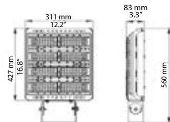
U-bracket
