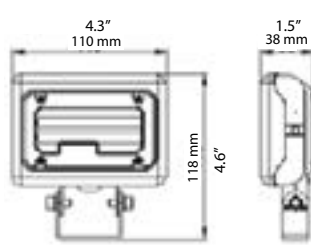
U-bracket
