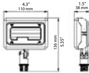
Knuckle
